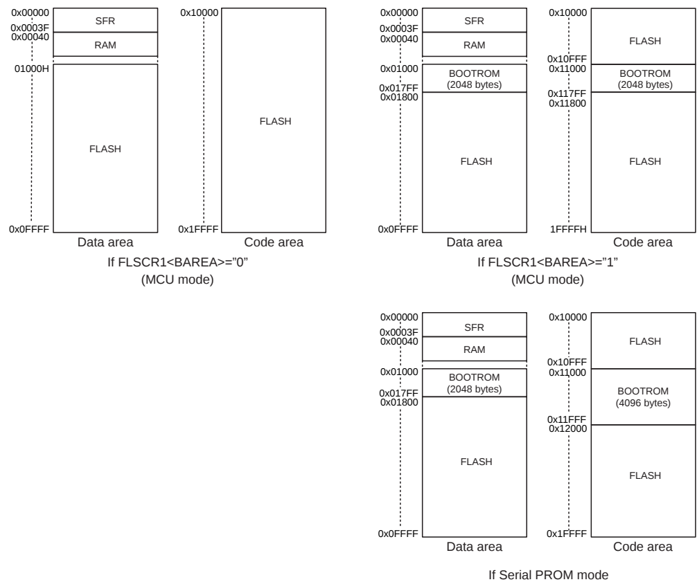
Figure 26-3 Memory Mapping
