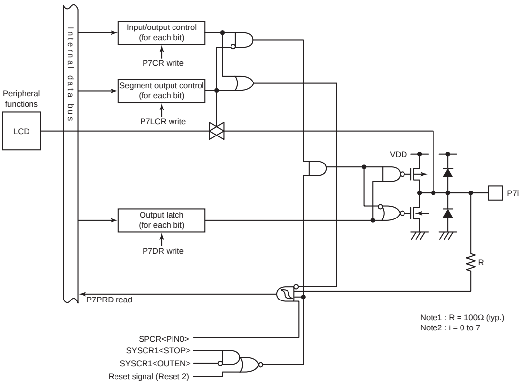
Figure 8-9 Port P7
