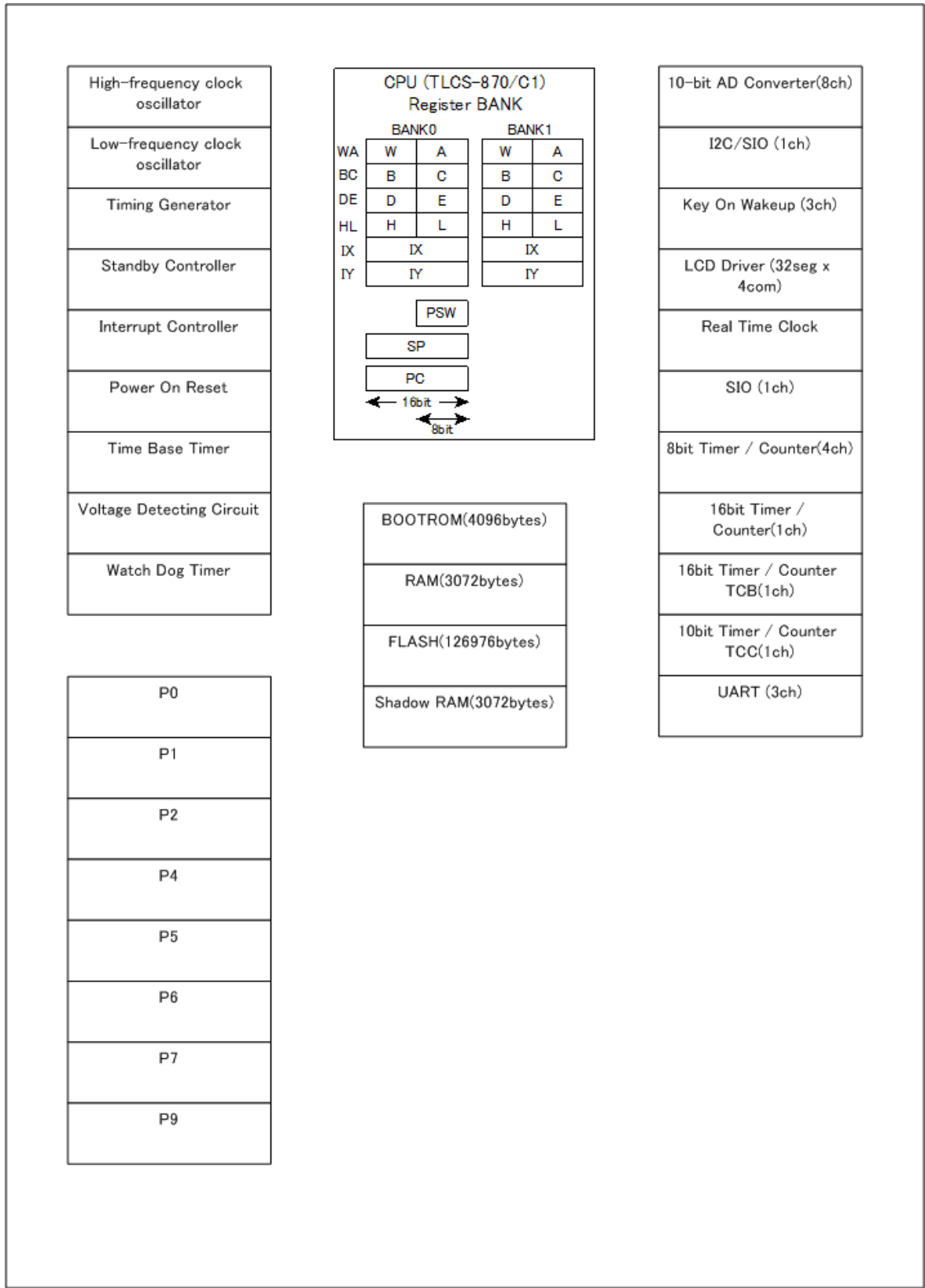
Figure 1-2 Block Diagram
