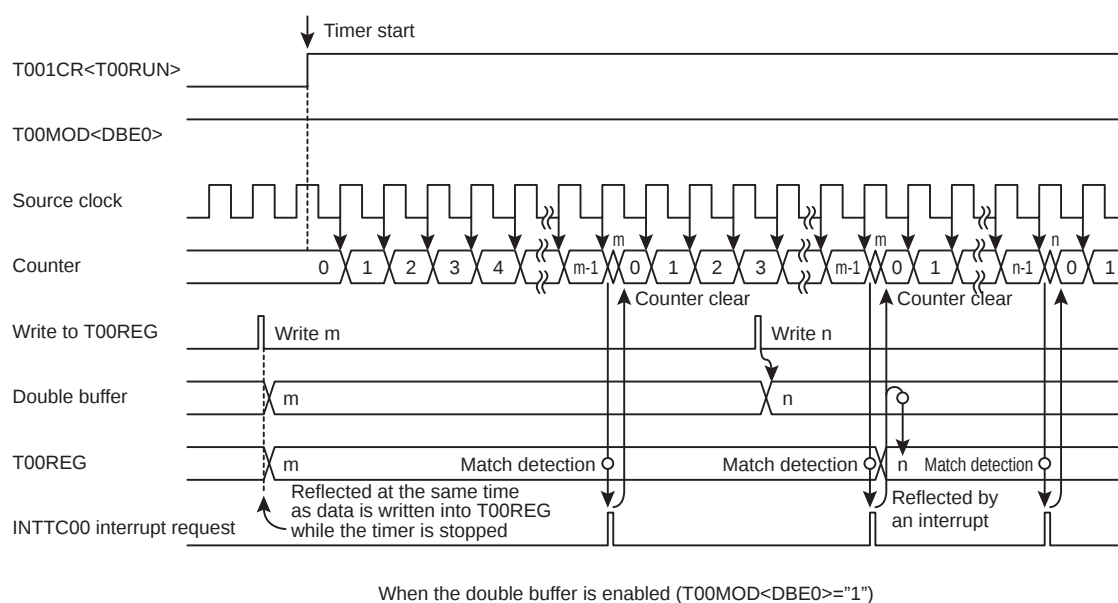
Figure 16-2 Timer Mode Timing Chart
