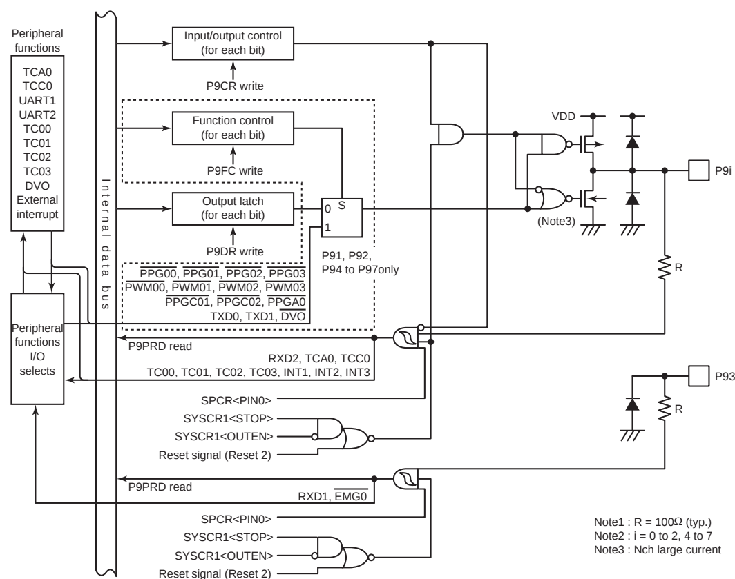
Figure 8-10 Port P9
