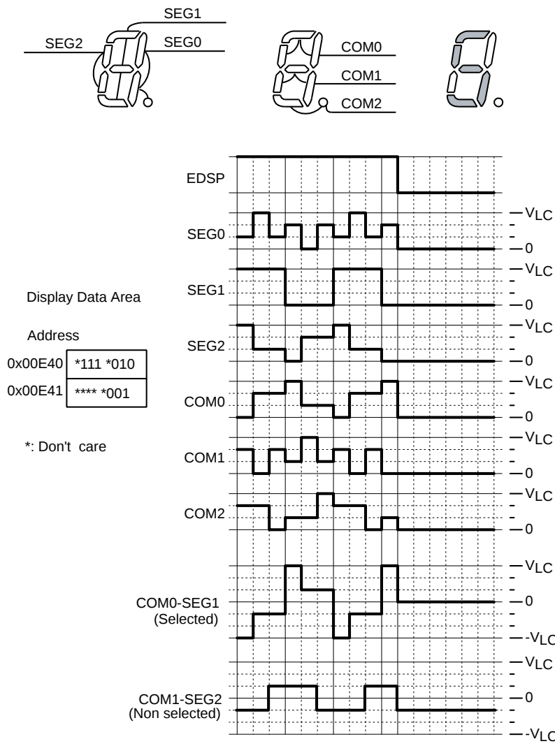
Figure 23-9 1/3 Duty (1/3 Bias) Drive
