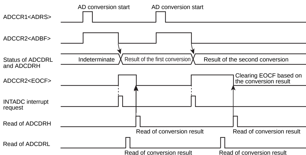
Figure 22-2 Single Mode
