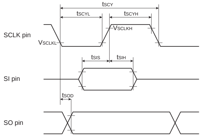
Figure 19-17 AC Characteristics
