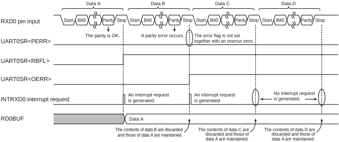
Figure 18-13 Framing/Parity Error Flags When an Overrun Error Occurs
