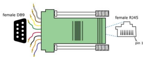
Figure 2-16. Female DB-9 to RJ-45 Adapter (green)
