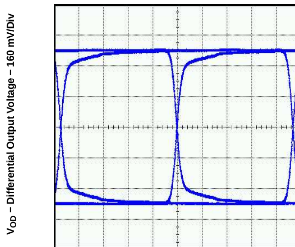
OUTPUT EYE-DIAGRAM AT 1.0625 GBPS AND MAXIMUM INPUT VOLTAGE ( 1200\text{ mV}_{p-p} )
