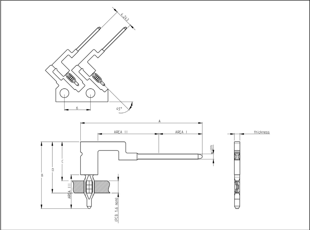
Product Drawing 1417081
