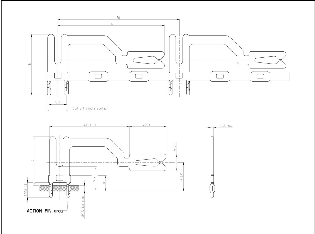
ACTION PIN Press-Fit Pin 90° Special Contact
