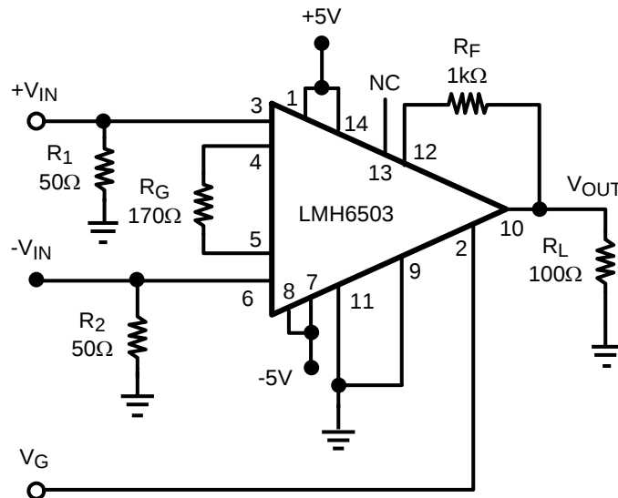
Figure 2. A_{VMAX} = 10V/V
