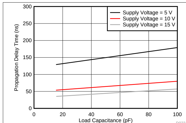
CLOCK or SET to Q, CLOCK or RESET to \bar{Q} Figure 5. Typical Propagation Delay Time vs Load Capacitance
