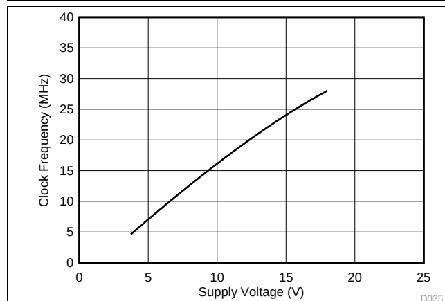
Figure 7. Typical Maximum Clock Frequency vs Supply Voltage
