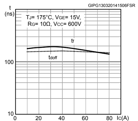
Figure 18. Switching time vs. collector current
