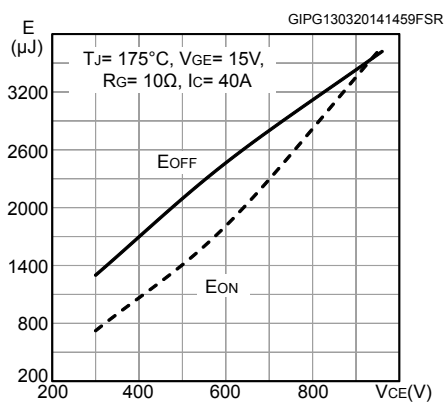
Figure 17. Switching energy vs. collector emitter voltage
