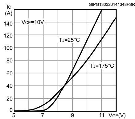
Figure 9. Transfer characteristics
