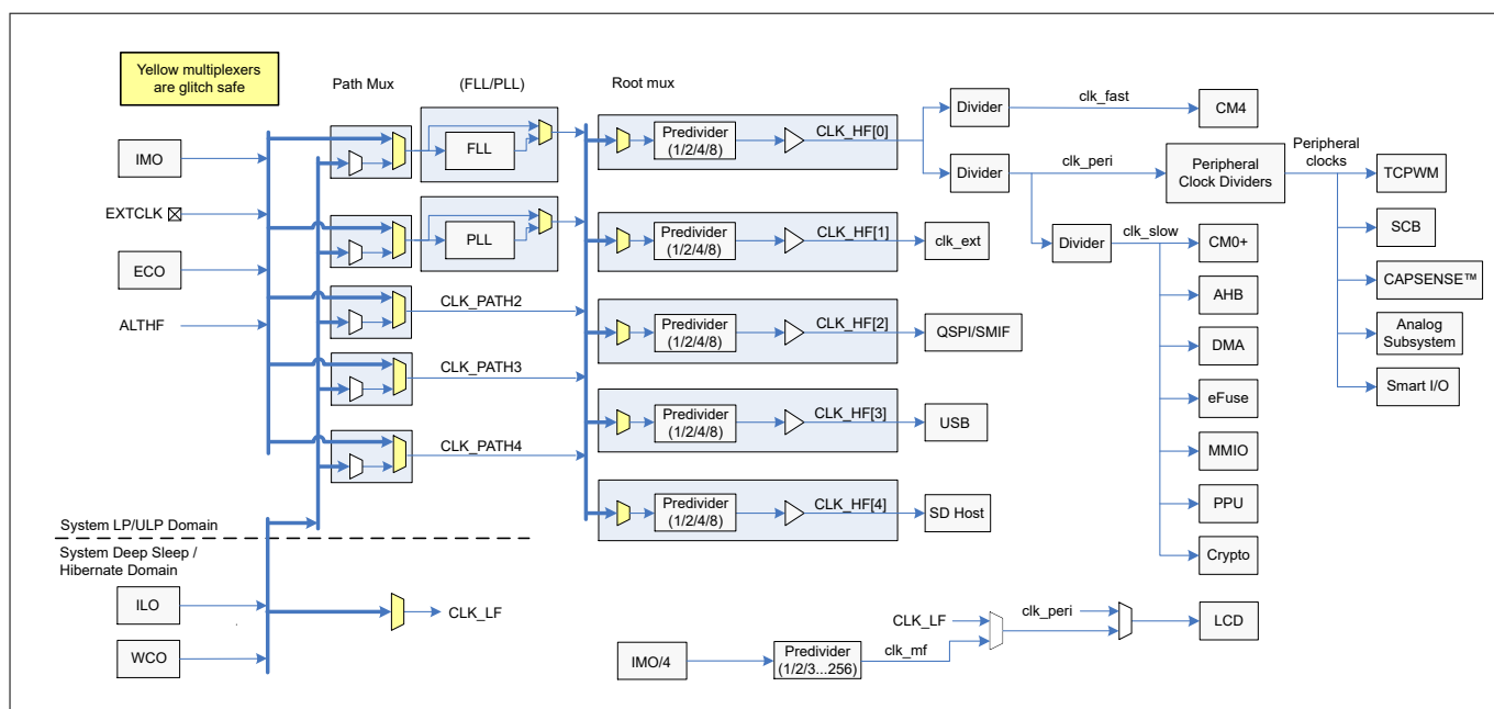
Figure 3 Clocking diagram
