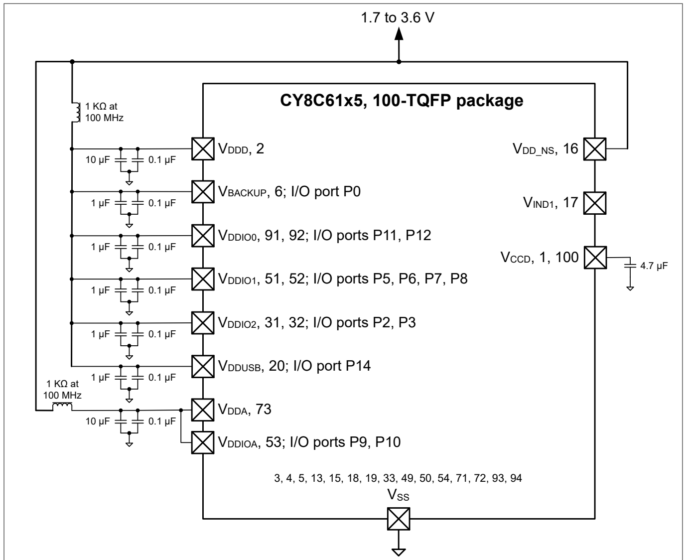
Figure 12 100-TQFP (No Buck) power connection diagram
