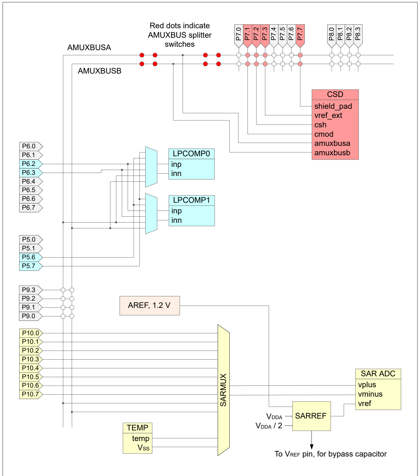
Figure 6 Analog subsystem
