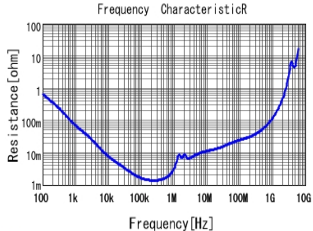
■ GRM32EB31A476ME20 R DC0V, 20degC
