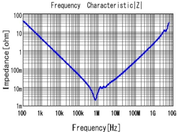
■ GRM32EB31A476ME20 |Z| DC0V, 20degC
