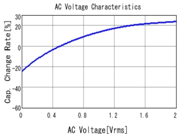
■ GRM32EB31A476ME20 C-AC Voltage capchange, DC0V, 20.0d
