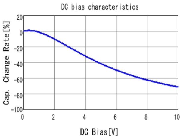
■ GRM32EB31A476ME20 C-DC bias capchange, 20.0degC, AC0.
