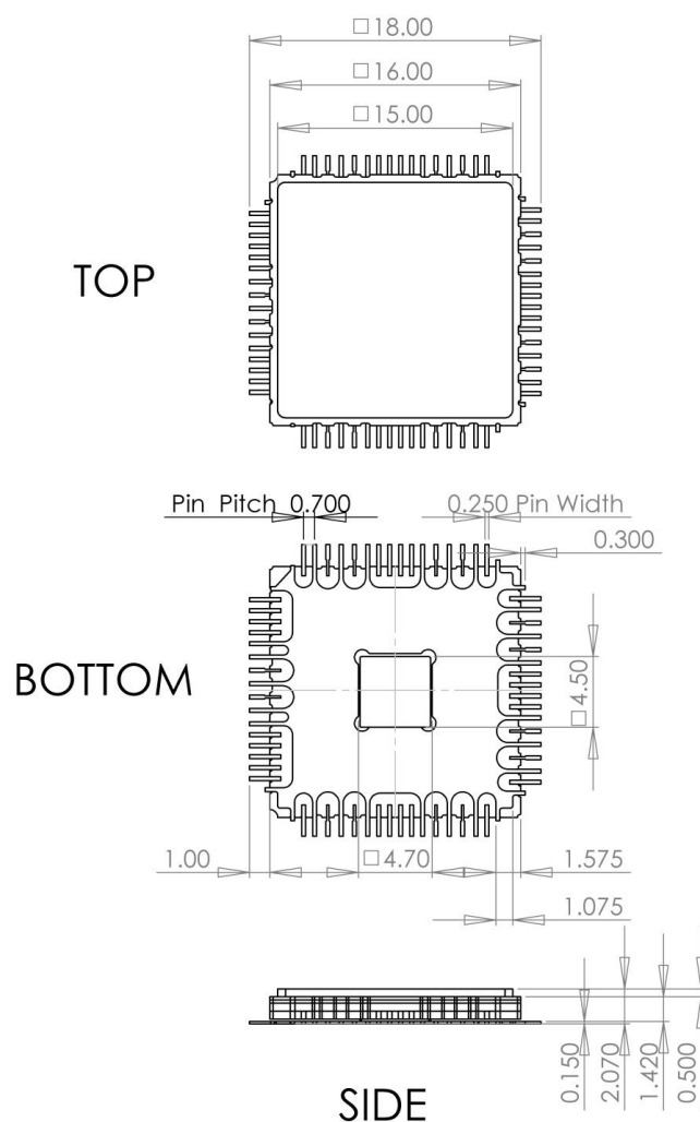
Fig. 3. Package Drawing
