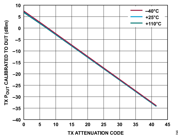
Figure 201. Transmitter Absolute Power vs. Transmitter Attenuation Code, Baseband Frequency = 18 MHz, Backoff = 0.2 dBFS
