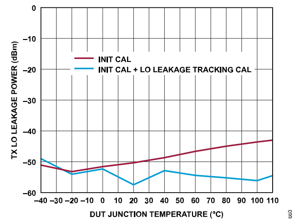
Figure 209. Transmitter LO Leakage Power vs. DUT Junction Temperature (Low to High), Baseband Frequency = 4 MHz, Backoff = 0.5 dBFS, Attenuation Code = 0
