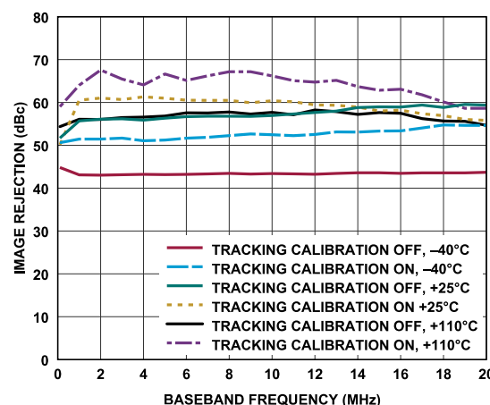
Figure 203. Transmitter Image Rejection vs. Baseband Frequency, Tracking Calibration On vs. Tracking Calibration Off, Transmitter Attenuation Code = 0
