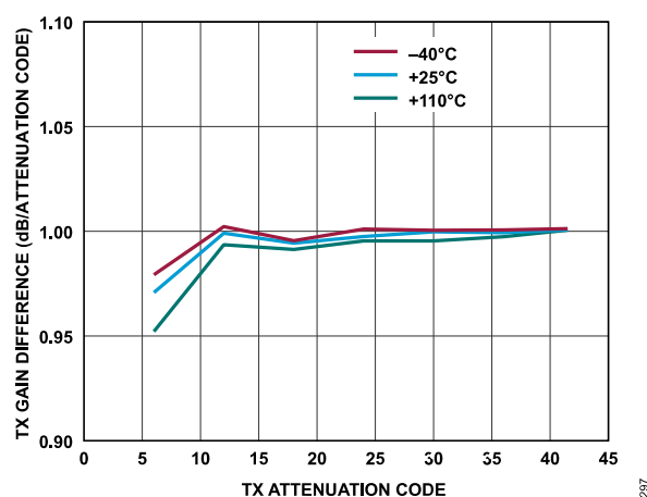
Figure 202. Transmitter Attenuation Delta (Error) vs. Transmitter Attenuation Code, Baseband Frequency = 18 MHz, Backoff = 0.2 dBFS
