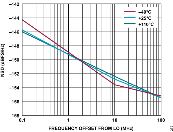
Figure 180. Transmitter NSD vs. Frequency Offset from LO, Baseband Frequency = 5.6 MHz, Transmitter Channel = Ch1
