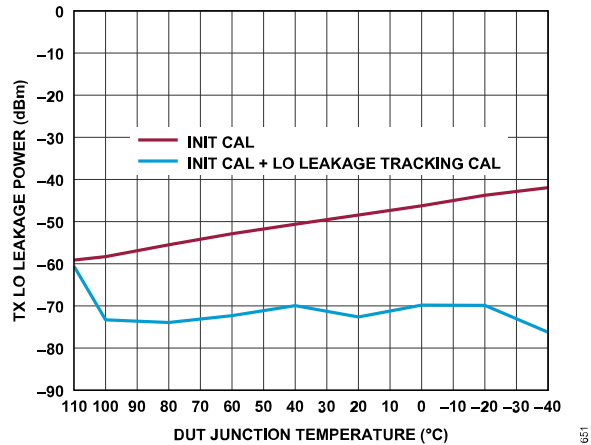
Figure 39. Transmitter LO Leakage Power vs. DUT Junction Temperature (High to Low), Baseband Frequency = 4 MHz, Backoff = 0.5 dBFS, Attenuation Code = 0
