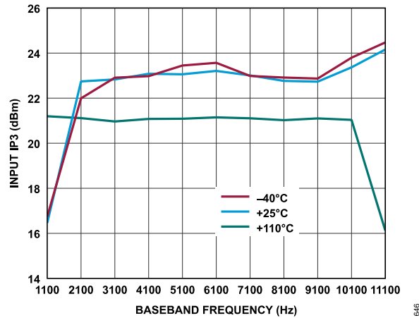
Figure 343. Receiver Input IP3 vs. Baseband Frequency, ADC = High Performance, f_1 = Baseband Frequency + 1 MHz, f_2 = Baseband Frequency + 2 MHz, Gain Index = 255, First-Order TIA with f_{1dB} = 4 MHz, P_{OUT} = -14 dBFS at -40°C and +25°C, P_{OUT} = -12 dBFS at +110°C
