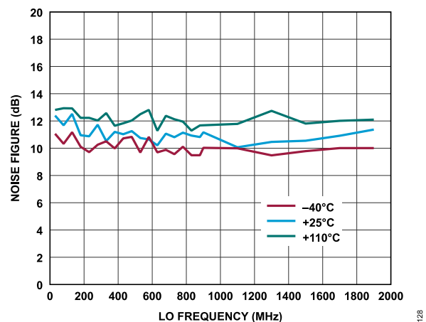
Figure 7. Receiver Noise Figure vs. LO Frequency, Baseband Frequency = 5.6 MHz, ADC = High Performance
