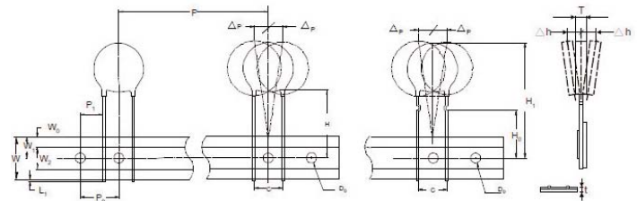
Figure 2 - PTR060V0250-PTR060V0375
