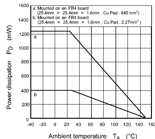
Fig. 8.6 P_D - T_a
