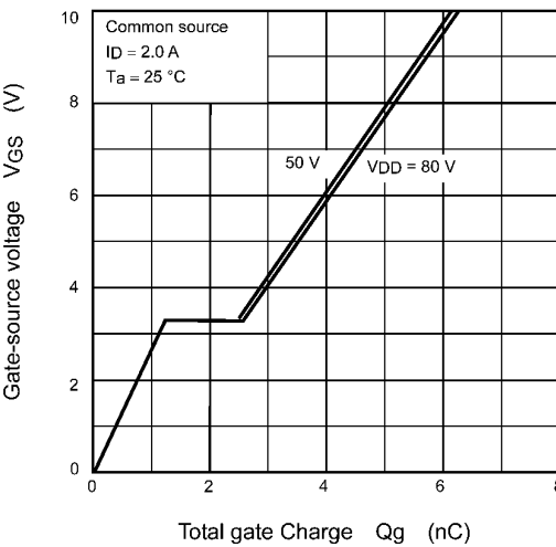
Fig. 8.5 Dynamic Input Characteristics
