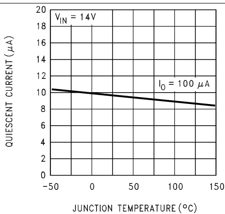
Figure 5. Quiescent Current
