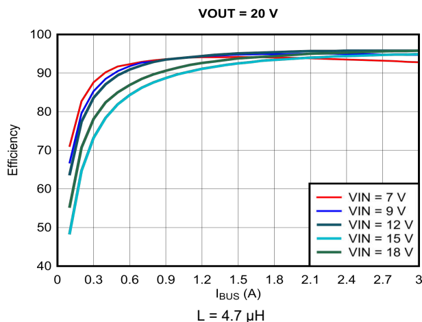
Figure 9-10. Efficiency vs Output Current ( I_{OUT} ), V_{OUT} = 20 V
