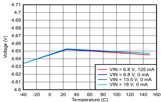
Figure 6-8. LDO_5V vs V_{IN} and Temperature
