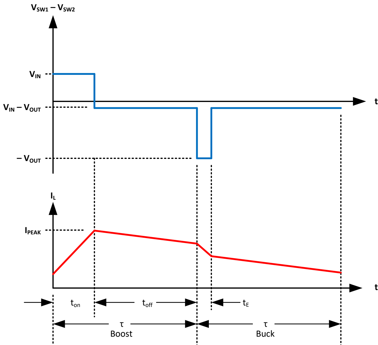
Figure 8-10. Boost Transition
