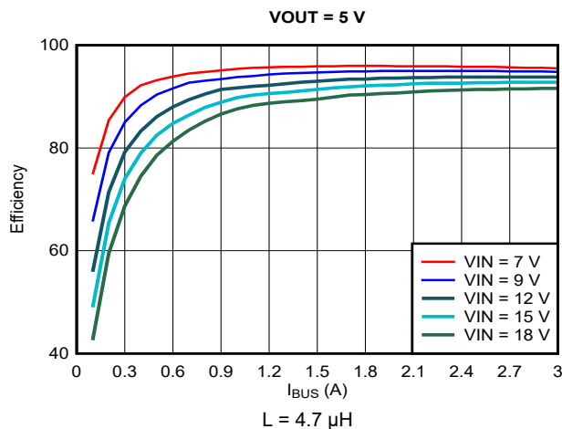
Figure 9-6. Efficiency vs Output Current ( I_{OUT} ), V_{OUT} = 5 V
