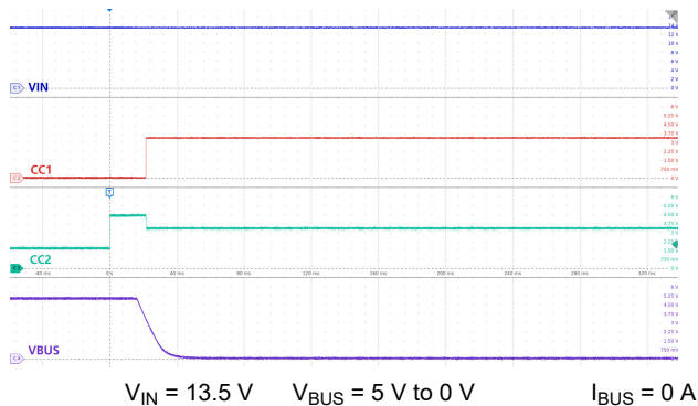
Figure 9-13. Type-C Detach
