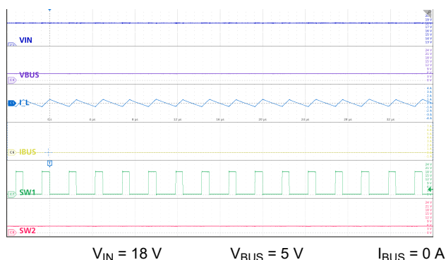
Figure 9-15. Buck Mode: High V IN , No Load
