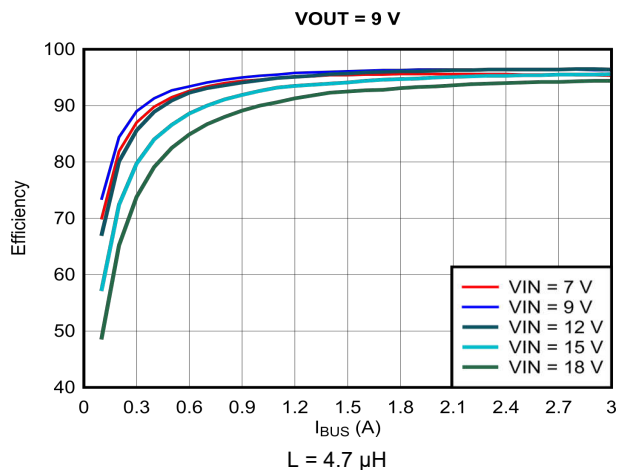
Figure 9-7. Efficiency vs Output Current ( I_{OUT} ), V_{OUT} = 9 V
