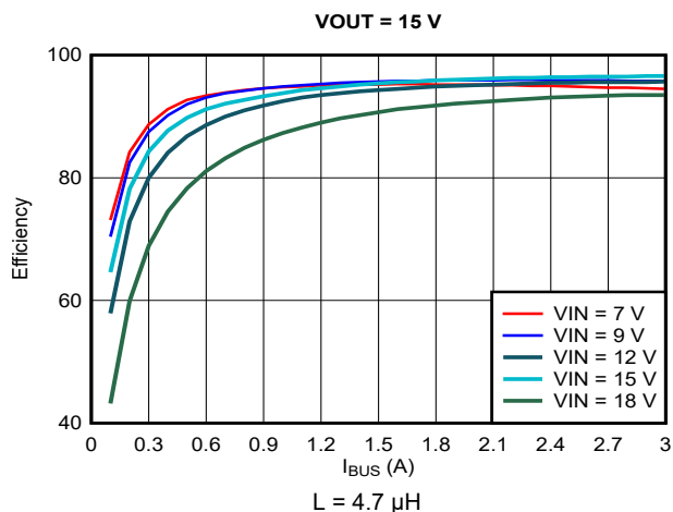
Figure 9-9. Efficiency vs Output Current ( I_{OUT} ), V_{OUT} = 15 V
