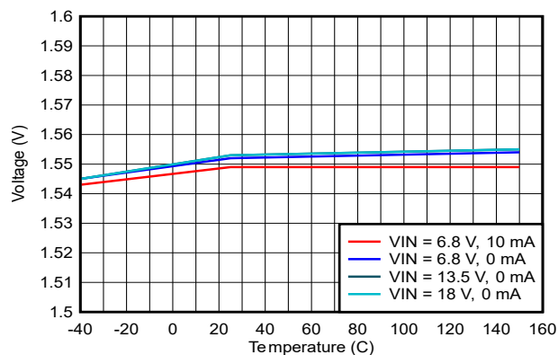
Figure 6-12. LDO_1V5 vs V_{IN} and Temperature
