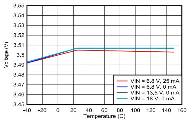
Figure 6-10. LDO_3V3 vs V_{IN} and Temperature
