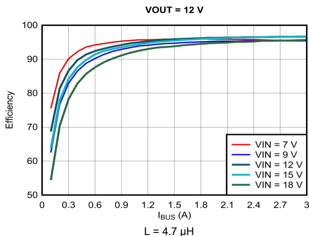
Figure 9-8. Efficiency vs Output Current ( I_{OUT} ), V_{OUT} = 12 V
