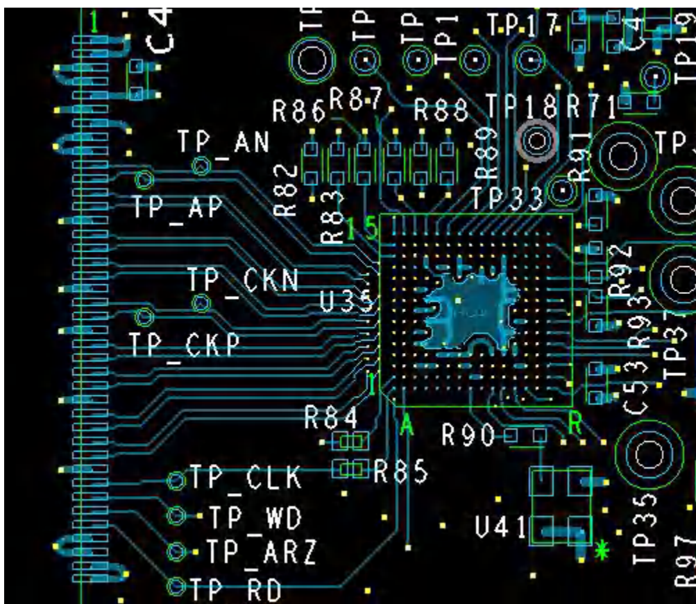
Figure 9-3. Layout Recommendation
