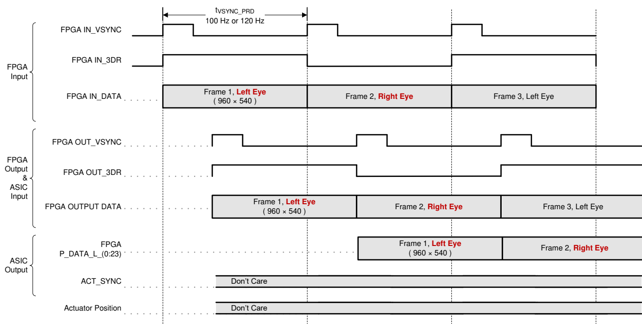
Figure 6-3. 3D Frame and Signal Timing
