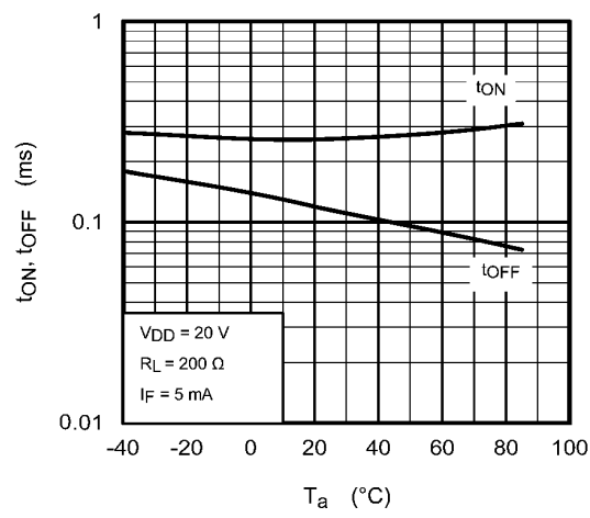
Fig. 14.8 t_{ON}, t_{OFF} - T_a
