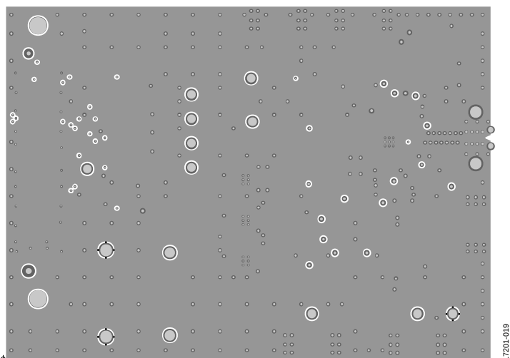
Figure 19. Layer 2 (Ground)
