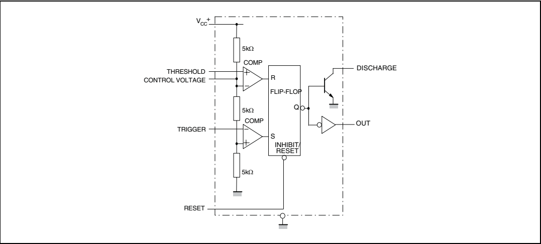
Figure 1. Block diagram
