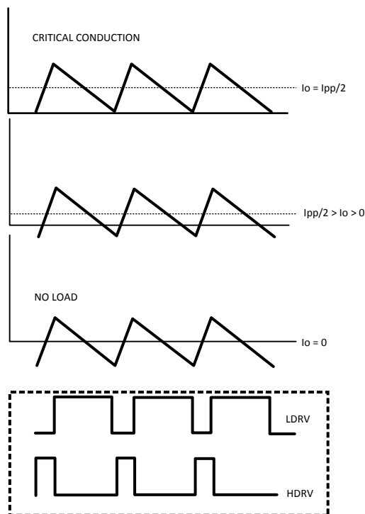
Figure 12. Inductor Current in FPWM Mode
