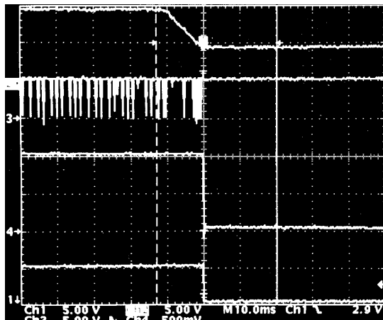
CH1: PGOOD, CH2: VIN, CH3: LDRV, CH4: Vo Output 1V @ 0.02A, VIN = 9.75V, FPWM, L = 10μH, f = 300kHz, C OUT = 660μF
