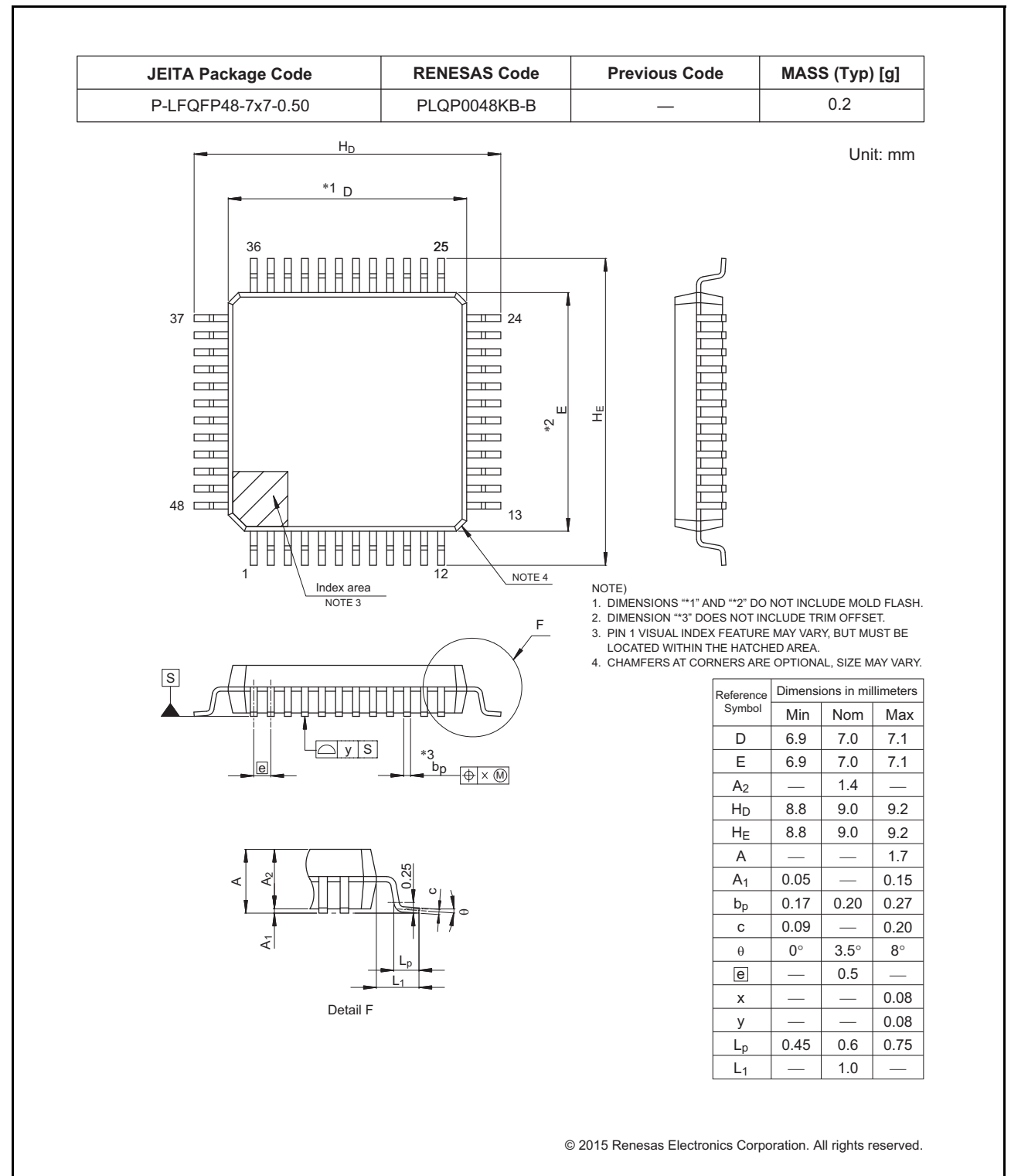
Figure 1.2 LQFP 48-pin
