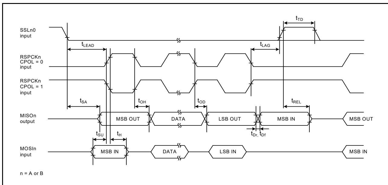
Figure 2.54 SPI timing (slave, CPHA = 0)
