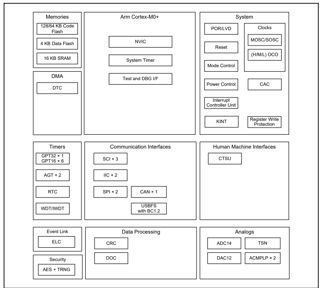
Figure 1.1 Block diagram
