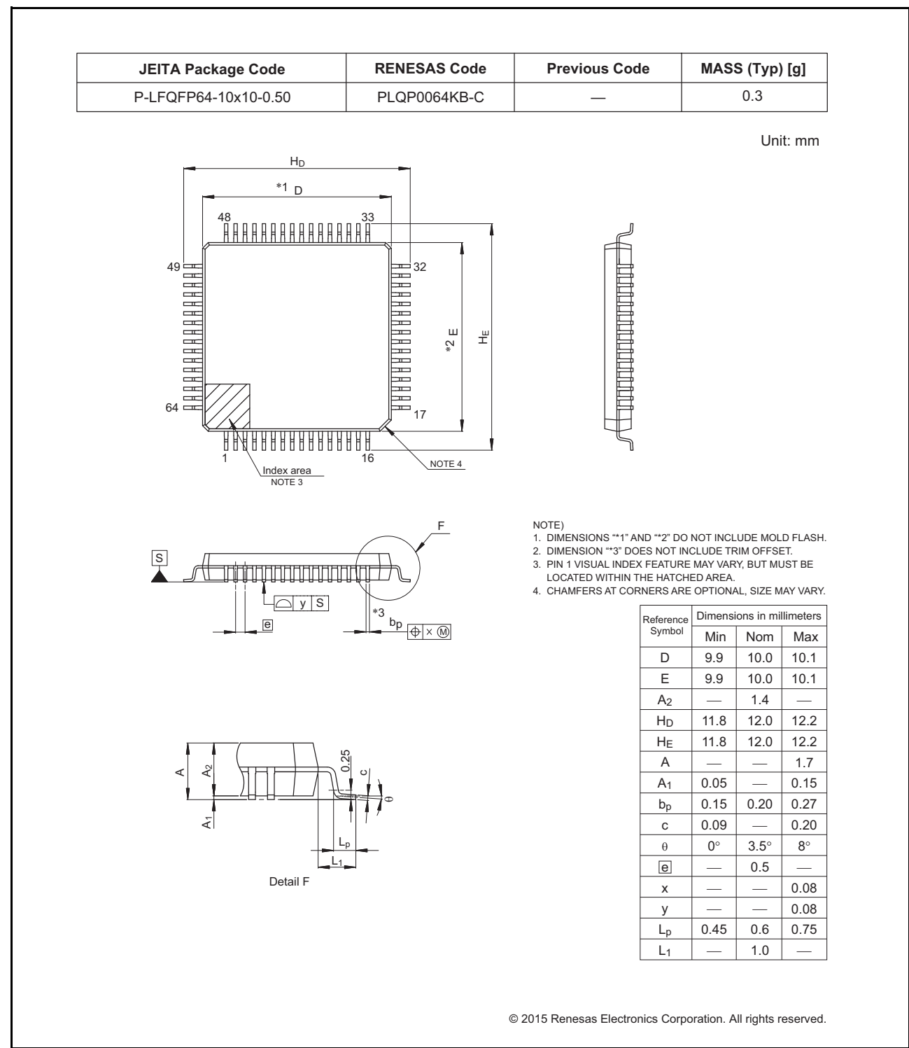
Figure 1.1 LQFP 64-pin
