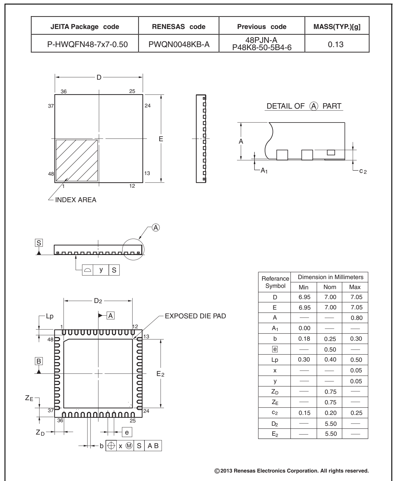
Figure 1.6 QFN 48-pin (1)
