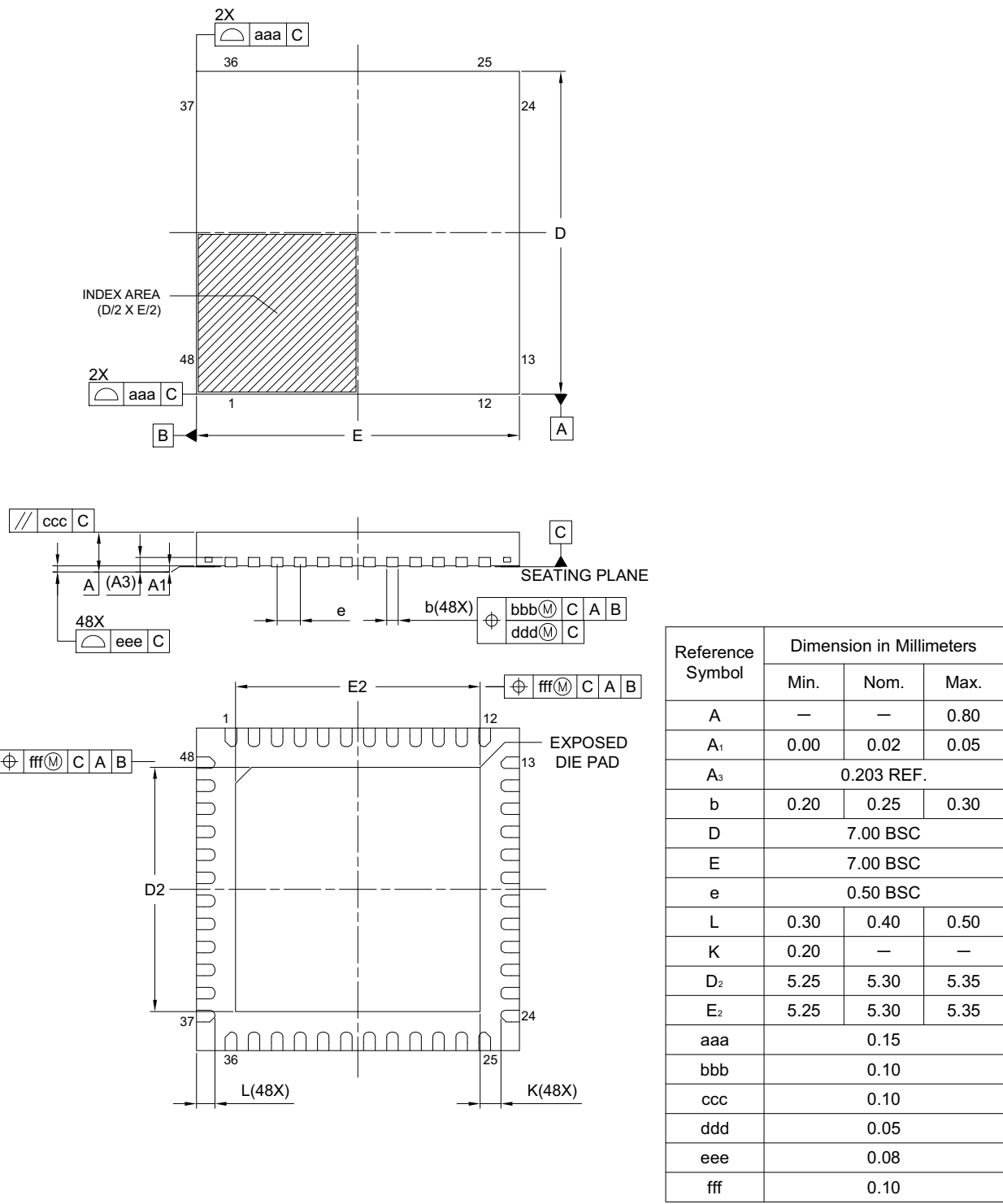
Figure 1.7 QFN 48-pin (2)
