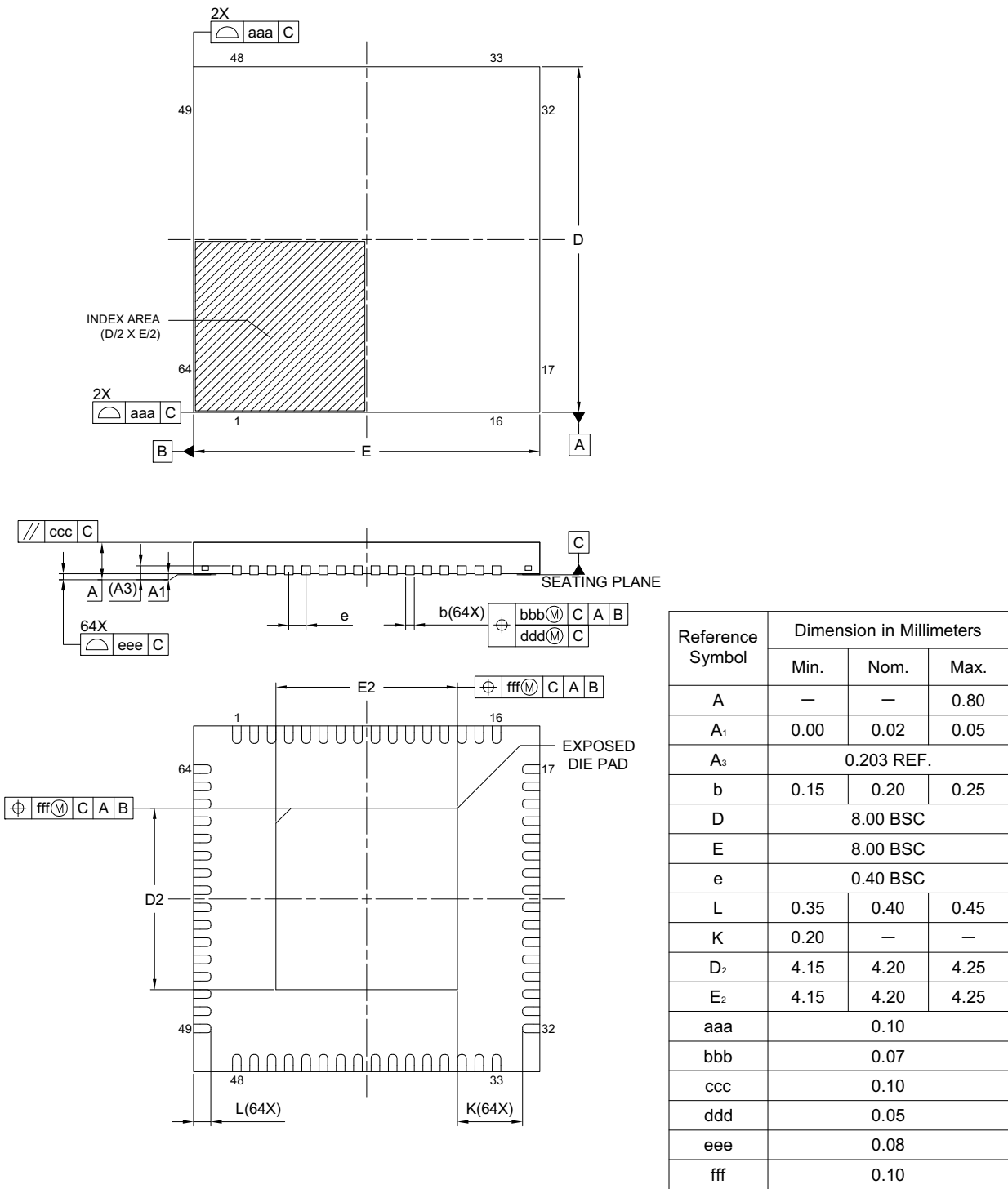
Figure 1.5 QFN 64-pin (2)
