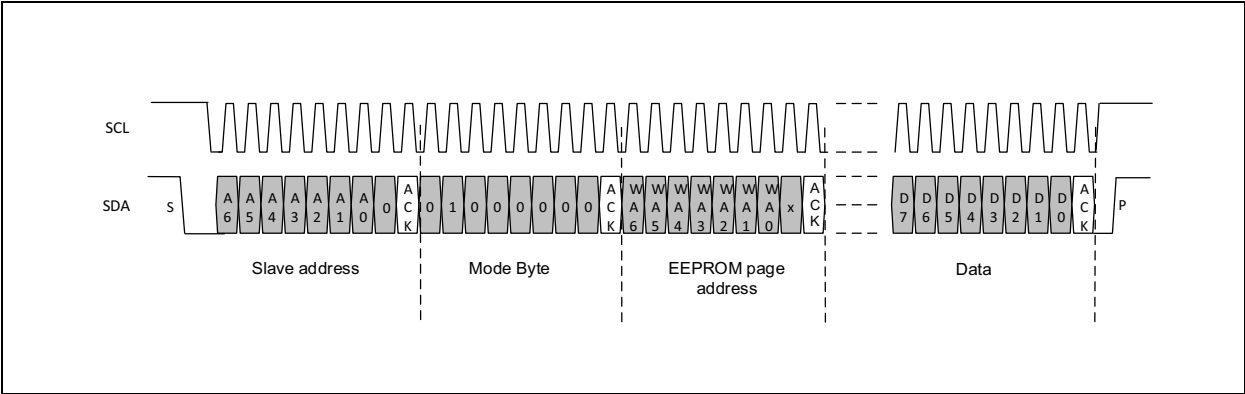
Figure 76: I 2 C Timing
