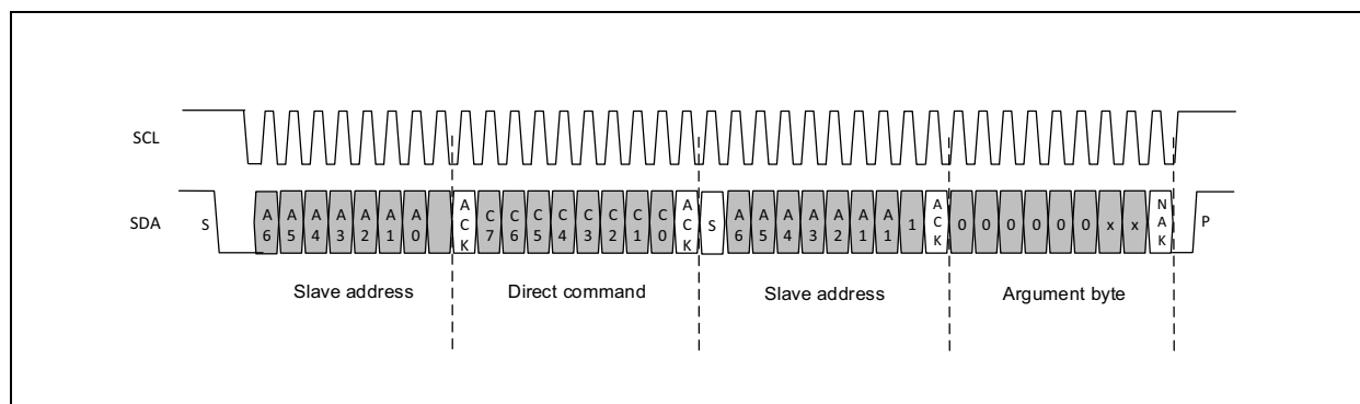
Figure 80: Sending a Direct Command over I 2 C
