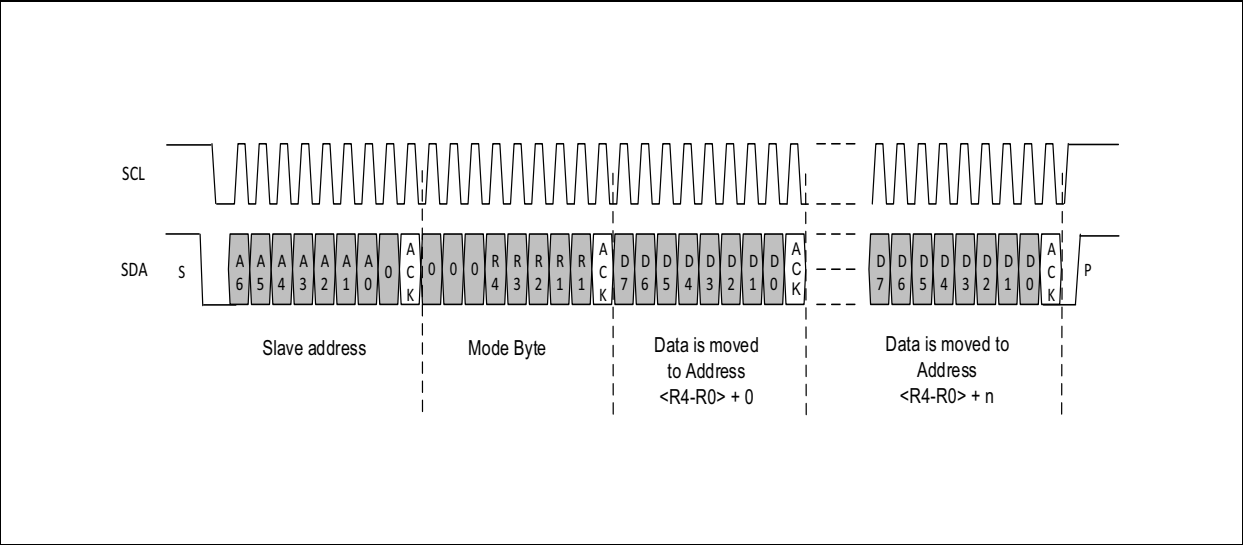
Figure 71: Writing Register Data with Auto-Incrementing Address over I 2 C
