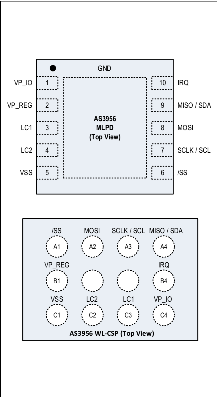
Figure 4: AS3956 Pin Diagram
