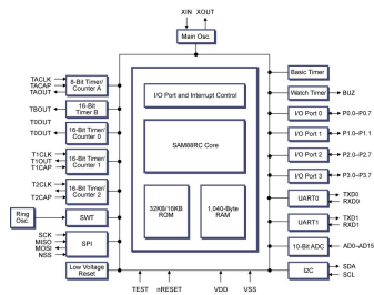
S3F8S35 MCU Block Diagram
