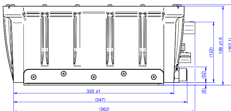
Figure 6. Side view
