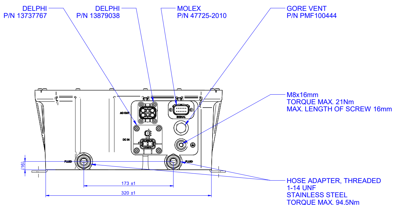
Figure 5. Front view
