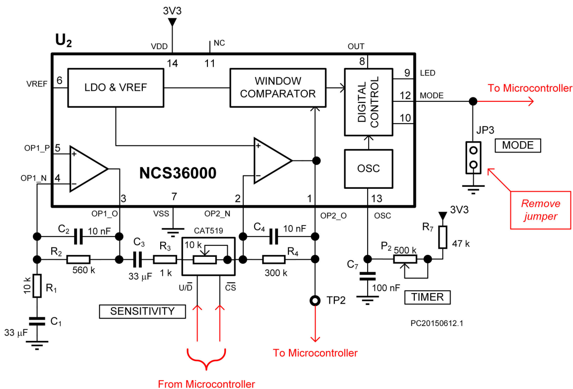
Figure 7. Schematic Diagram
