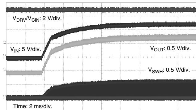
Startup with V_{IN} Ramping up V_{IN} = 12\text{ V} , V_{OUT} = 1.2\text{ V} , F_{SW} = 500\text{ kHz}
