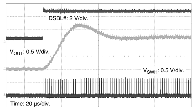
Startup with DSBL# Toggle High V_{IN} = 12\text{ V} , V_{OUT} = 1.2\text{ V} , F_{SW} = 500\text{ kHz}
