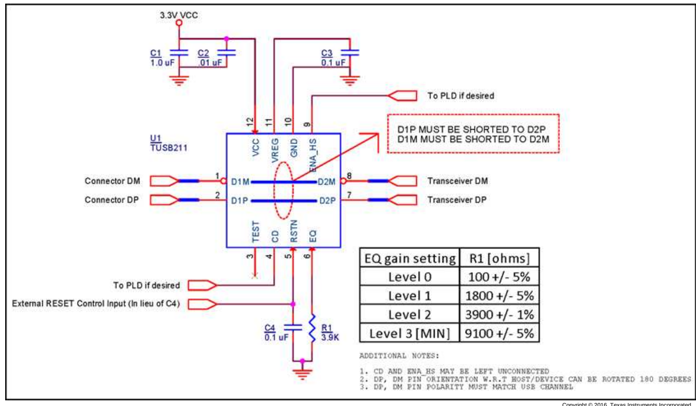
Figure 1. Reference Schematic
