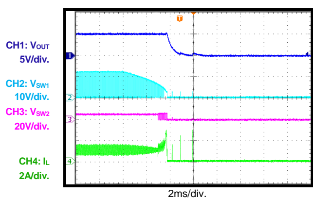
V_{IN} Power Off Load = 1A
