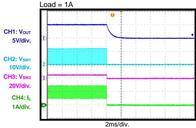
ENPWR Bit Disable through I 2 C Command Load = 1A
