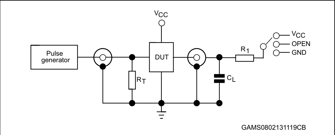
Figure 7. Test circuit
