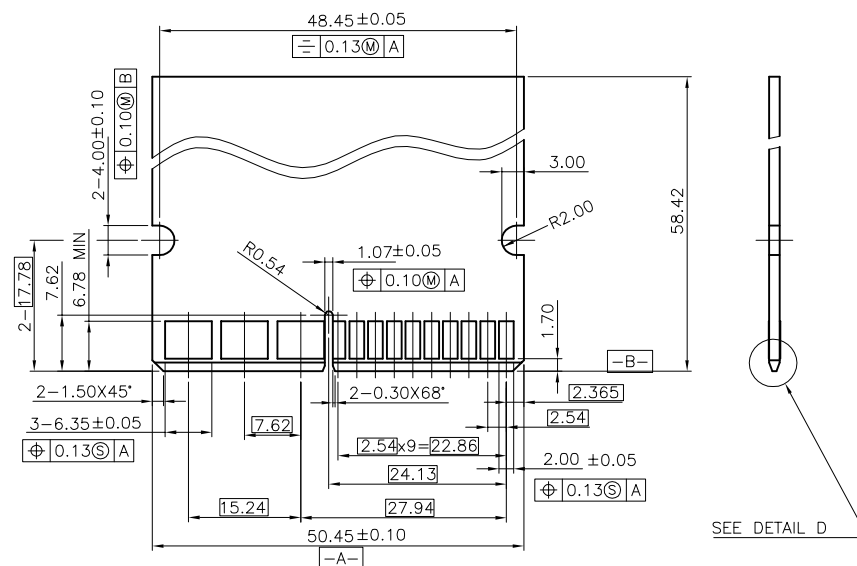
RECOMMENDED MATING BOARD EDGE CONFIGURATION
