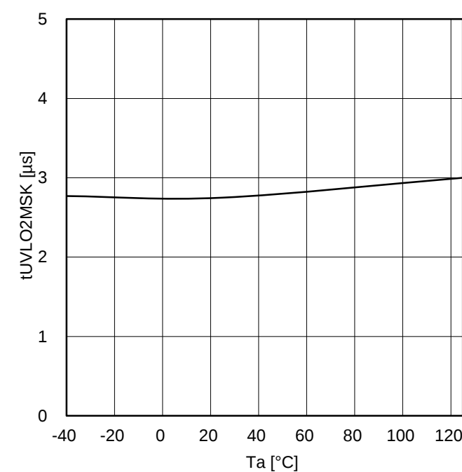
Figure 36. Output Side UVLO Mask Time vs Temperature
