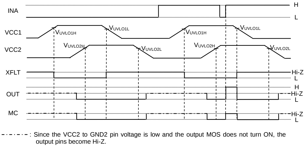
Figure 7. Power Supply Startup / Shutoff Sequence
