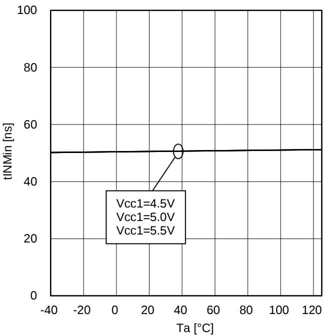
Figure 22. Logic (INA) Input Minimum Pulse Width vs Temperature
