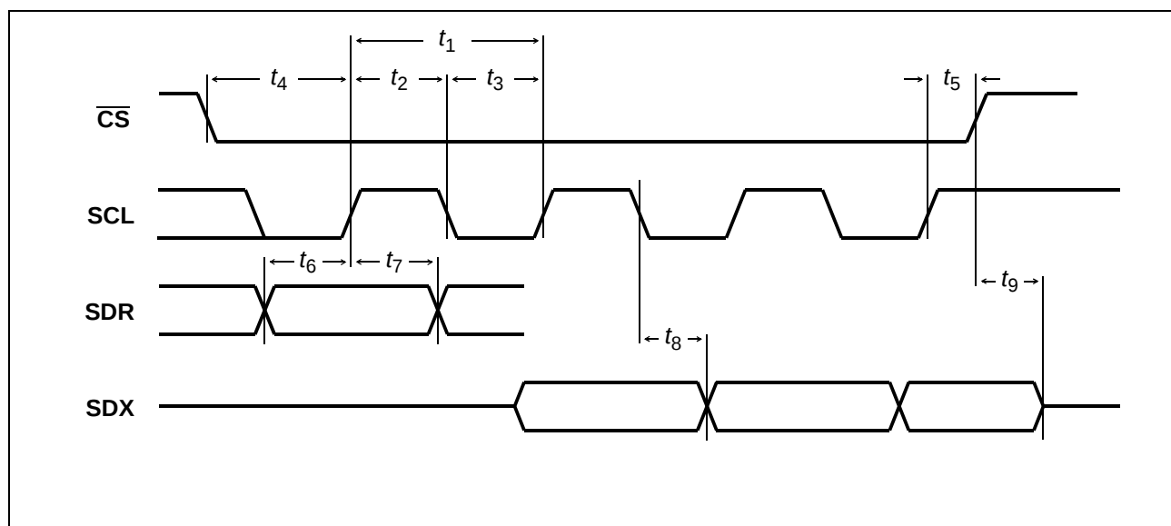
Figure 87 SCI Interface
