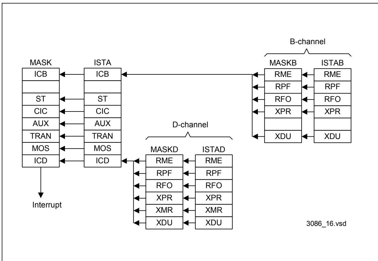
Figure 79 Interrupt Status Registers of the HDLC Controllers
