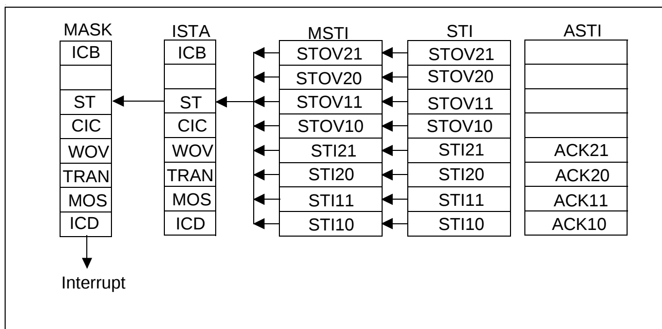
Figure 54 Interrupt Structure of the Synchronous Data Transfer
