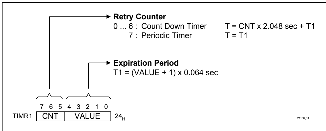
Figure 11 Timer 1 Register
