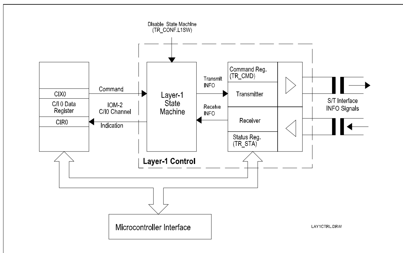
Figure 37 Layer-1 Control
