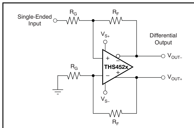
Figure 35. Single-Ended Input to Differential Output Amplifier
