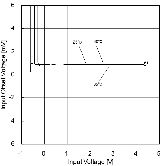
Figure 14. Input Offset Voltage vs Input Voltage ( V_{DD}=5V )
