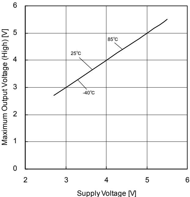
Figure 4. Maximum Output Voltage (High) vs Supply Voltage ( R_L=2k\Omega )
