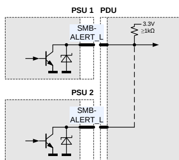
Figure 11. SMB_ALERT_L Connection
