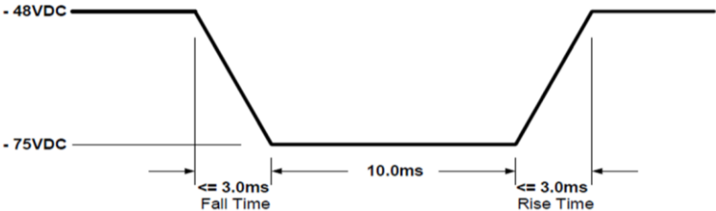
Figure 3. Minus 75 VDC Line Transient Test
