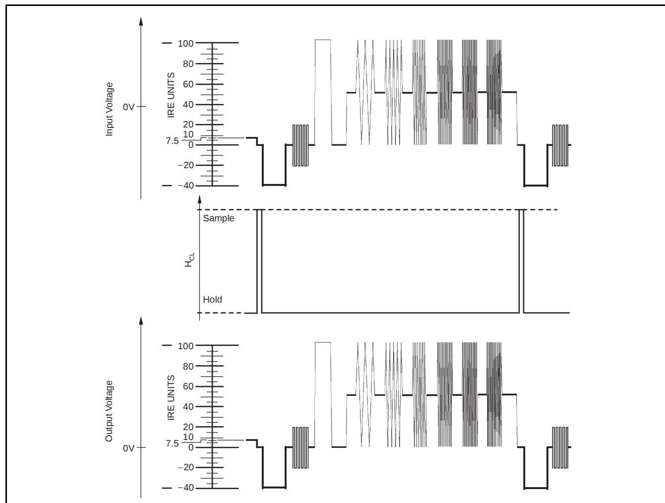
Figure 43. DC-Restore Timing
