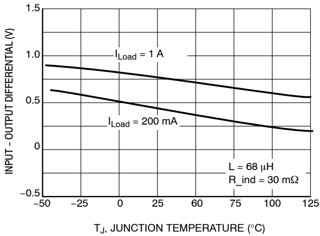
Figure 5. Dropout Voltage
