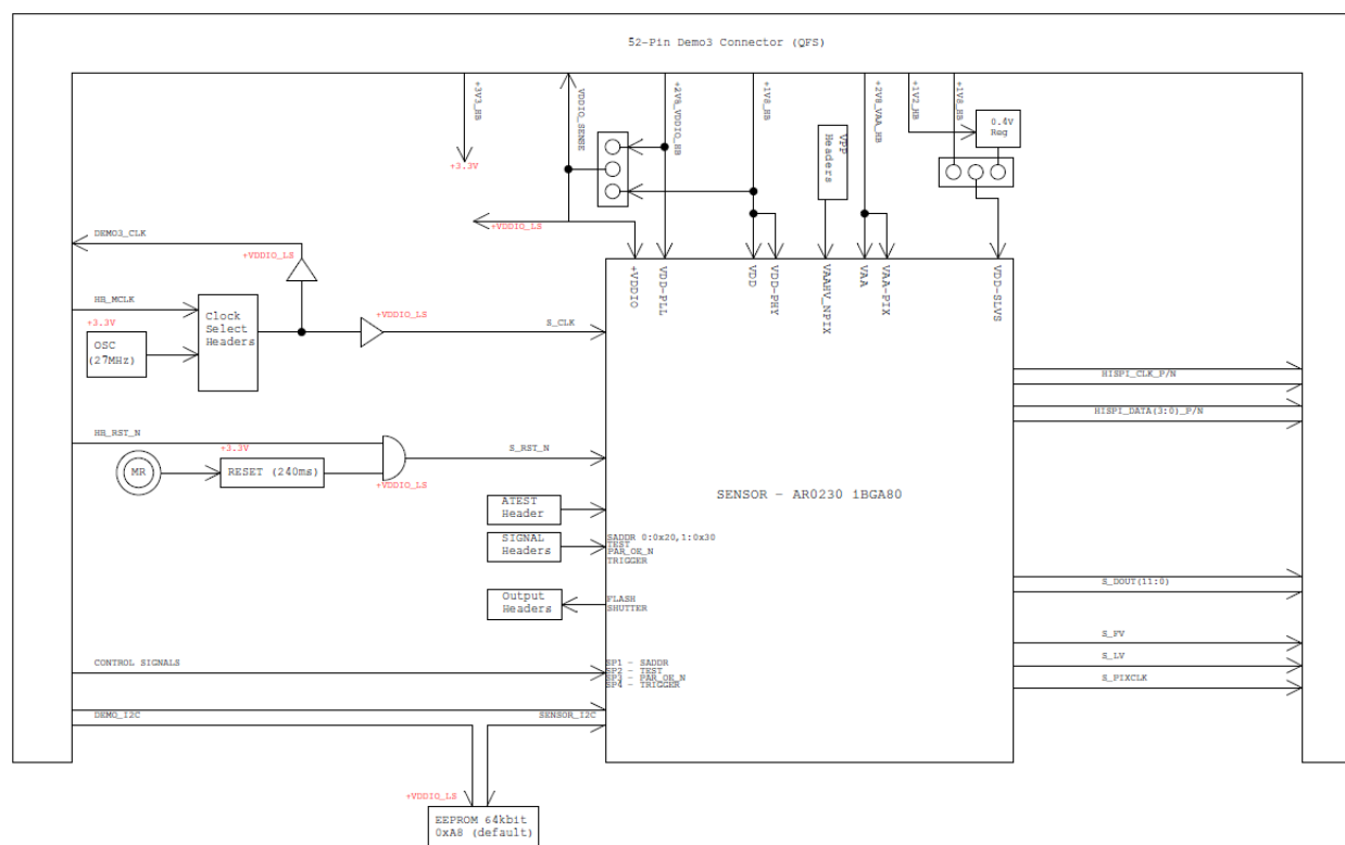
Figure 2. Block Diagram of AR0230ATSC00XUEAH3-GEVB
