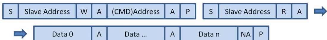
Figure 5. The I2C Command Format in AP43781
