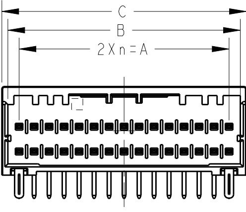
30POS(X-KEY): 1-2271888-5
