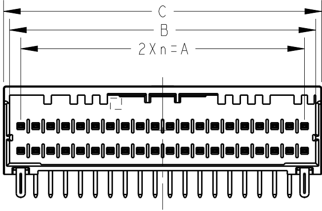
40POS(X-KEY): 1-2271888-0
