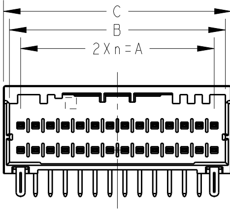
28POS(X-KEY): 1-2271888-4
