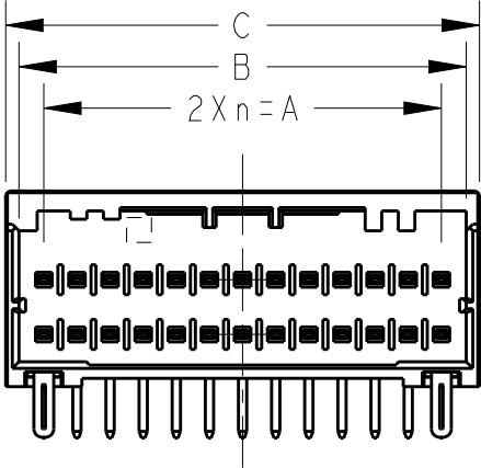
26POS(X-KEY): 1-2271888-3
