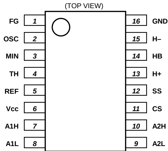
Fig.1 Pin configuration
