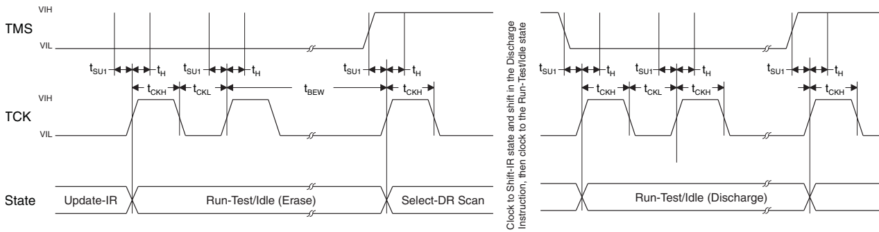
Figure 10. Programming Timing Diagram
