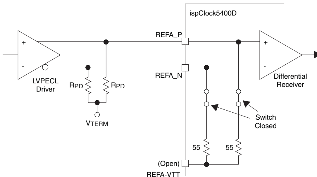
Figure 17. LVPECL Input Receiver Configuration
