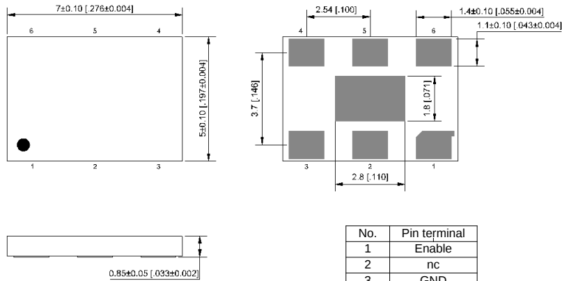
External Dimensions
