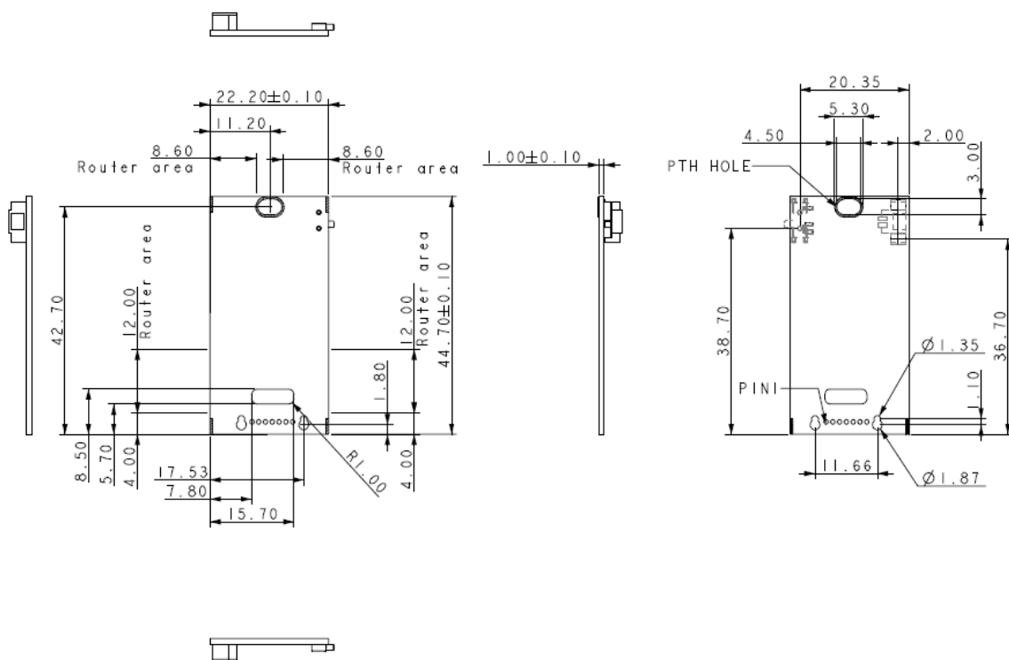
Power Cable (Unit: mm)
