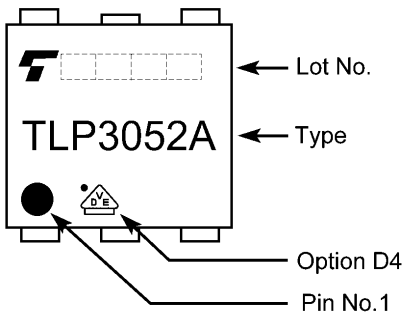
Fig. 16.3 Marking Example of TLP3052A (Note)
