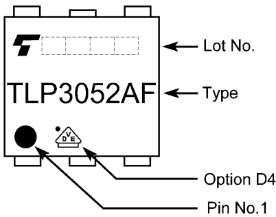
Fig. 16.4 Marking Example of TLP3052AF (Note)
