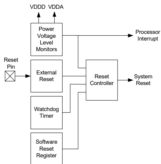
Figure 6-8. Resets
