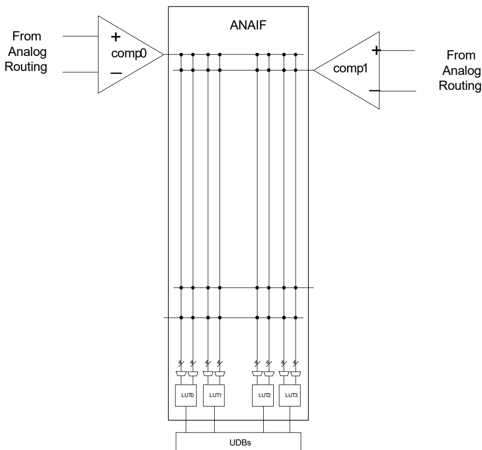
Figure 8-5. Analog Comparator
