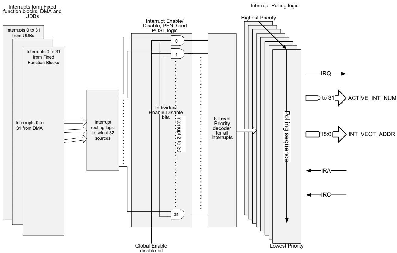
Figure 4-3. Interrupt Structure
