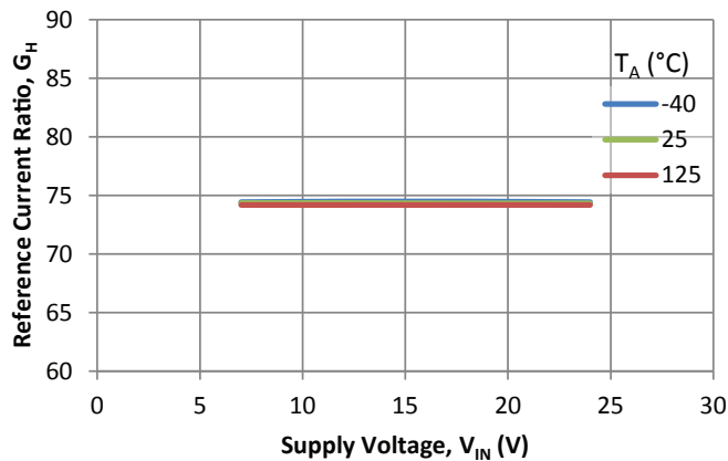
G_H vs. V_{IN} ( I_{REF} = 2 mA)
