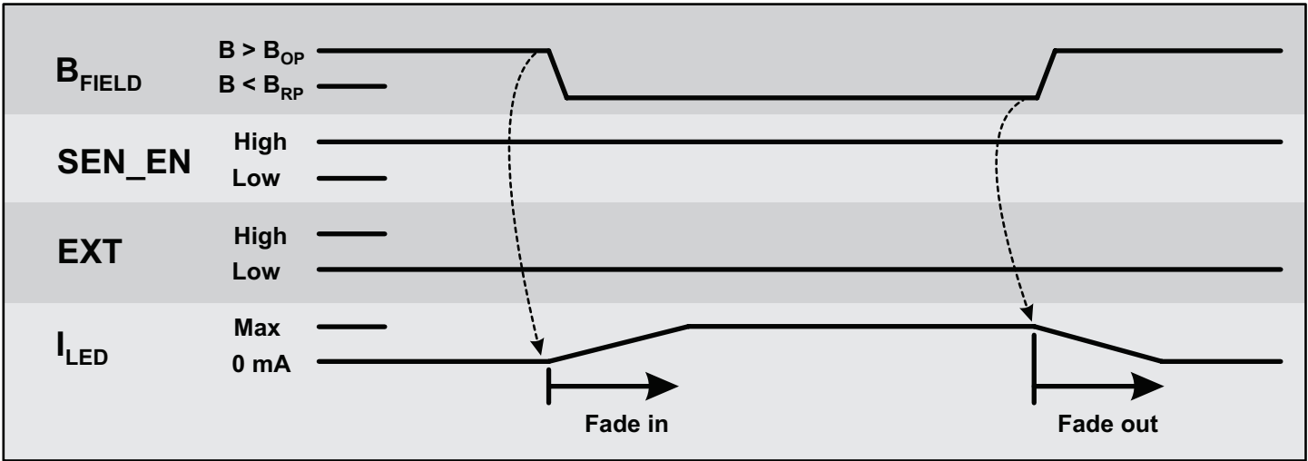
Figure 3: Hall-Activated Operation
