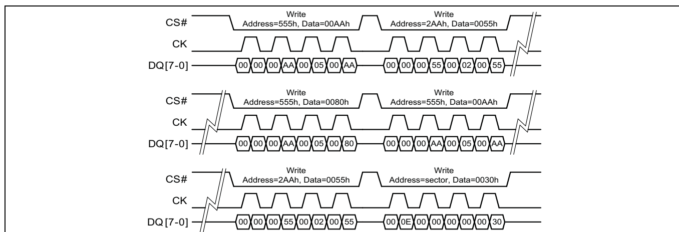
Figure 11 Write transaction usage example: Erase operation command sequence [24, 25, 26, 27]
