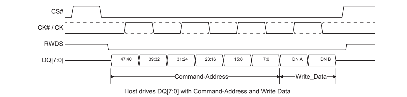
Figure 10 Write operation [21, 22, 23]
