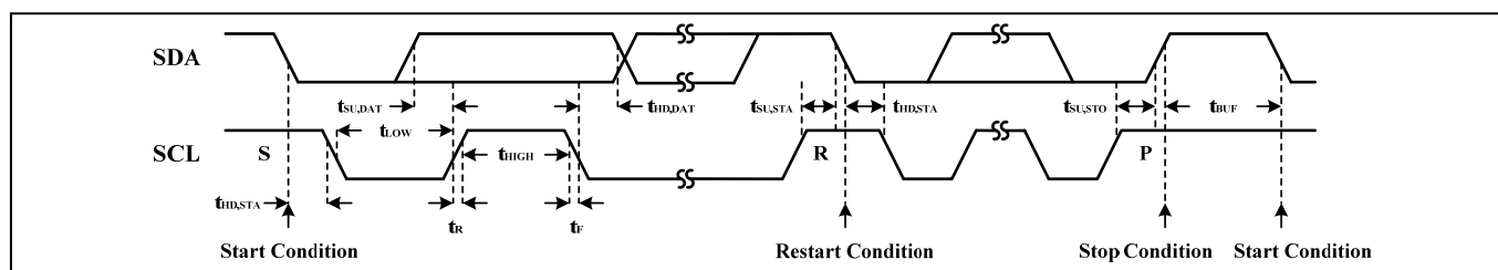
Figure 3 Interface Timing
