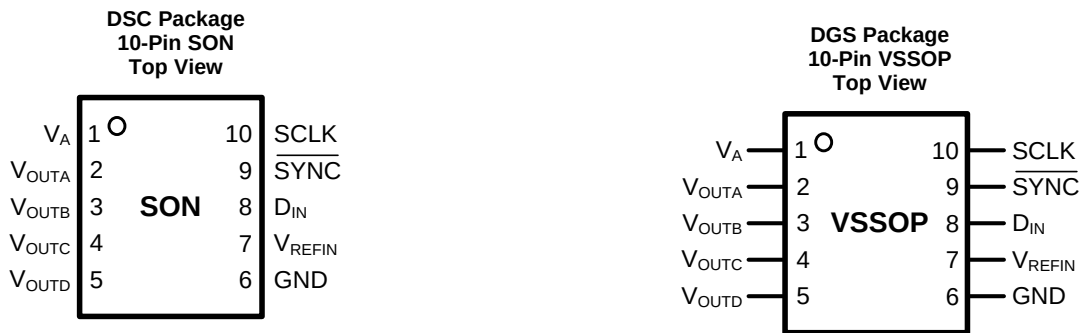
Pin Functions
